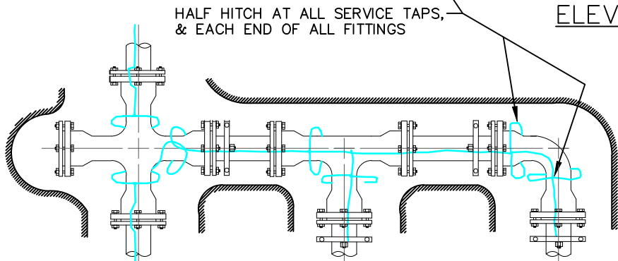
PLAN VIEW SHOWING TRACE WIRE AROUND FITTINGS
