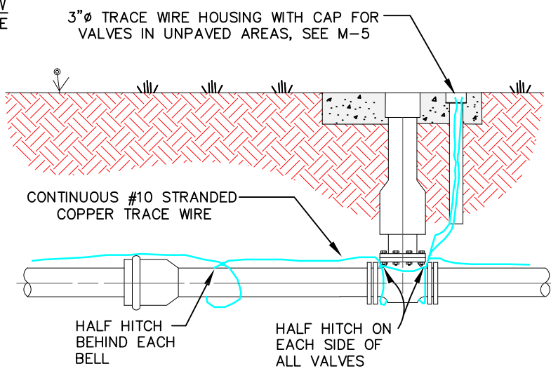
ELEVATION-VALVE BOX DETAIL
