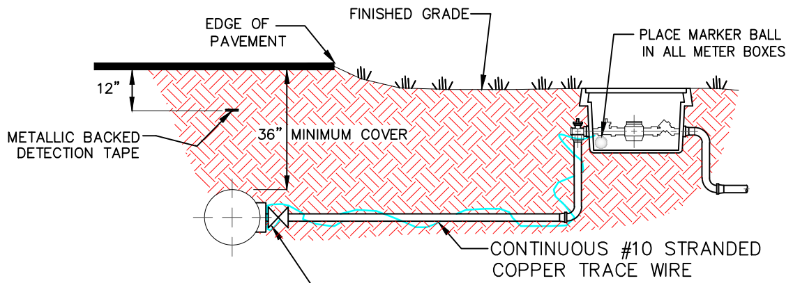
ELEVATION-SERVICE DETAIL
