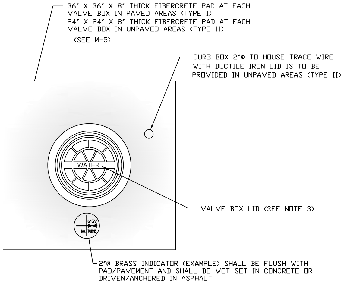
PLAN VIEW
