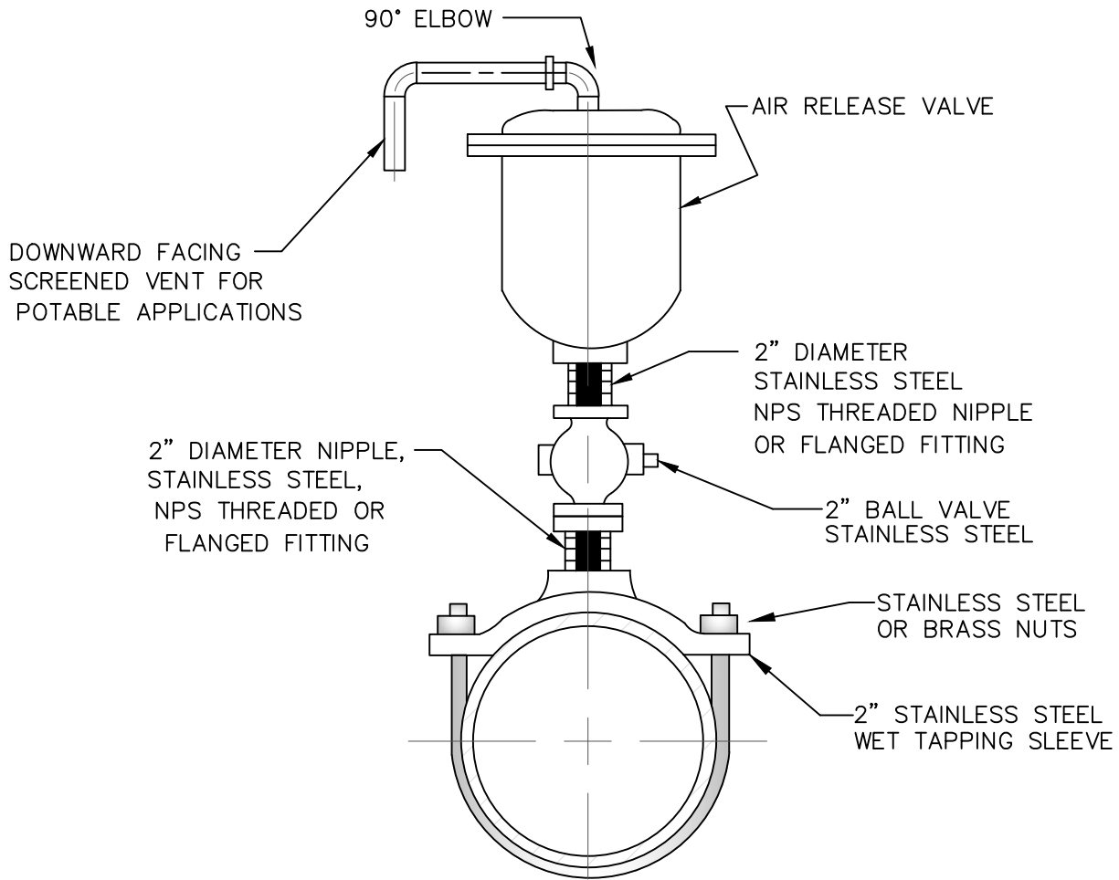
ELEVATION WATER MAIN/WASTEWATER MAIN
